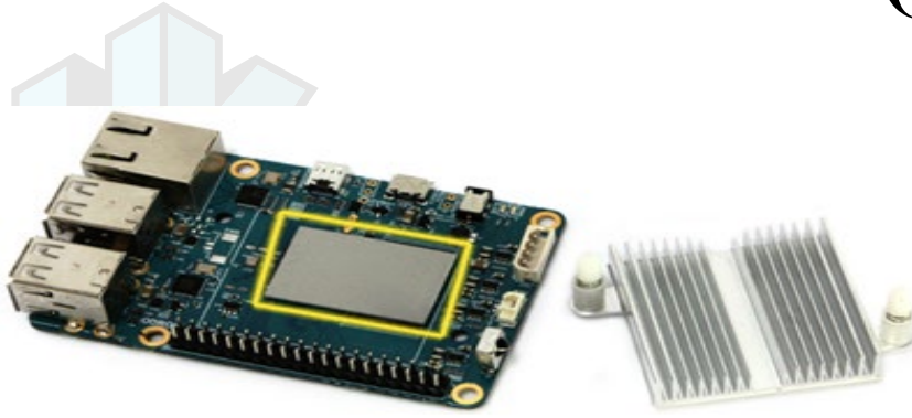
Heatsink thermal pad applied
